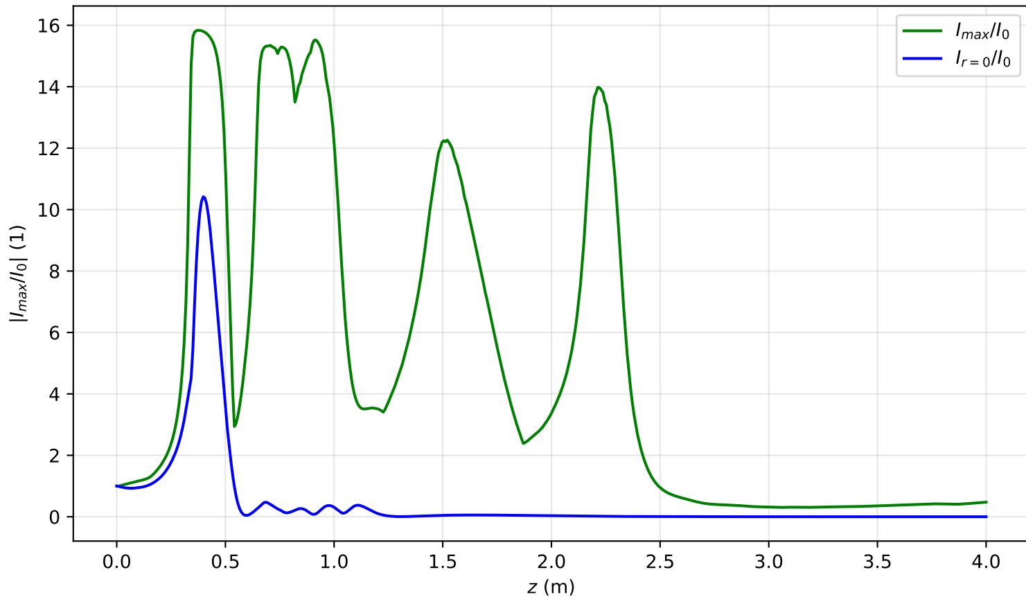
I_{max}(x=0, y=0, z)/I_0 , Pin=7.0Pcr, noisy input, artificial time
